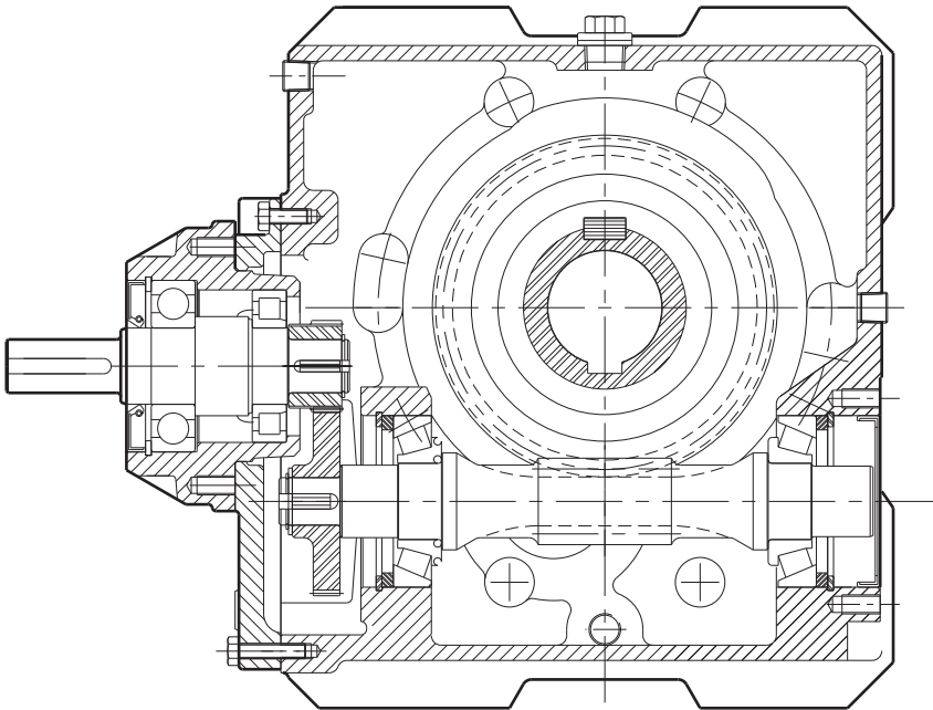
Hollow output shaft unit showing standard metric extension on input shaft adaptor
